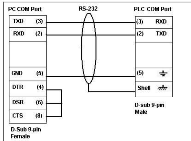
PGMCBL: Programming Cable Wiring
