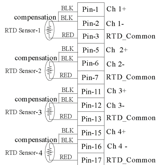
Equivalent Input Circuit
